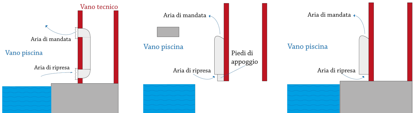
DUCT INSTALLATION
